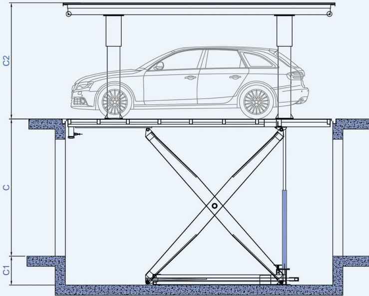
Section View-UP
