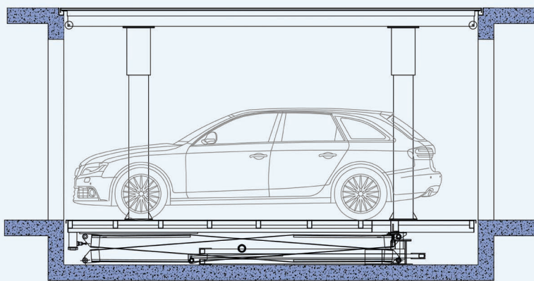
Section View-DOWN
