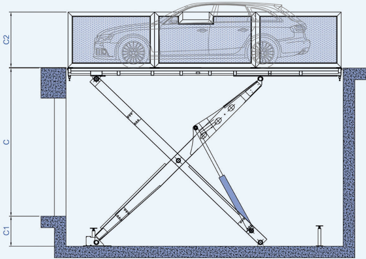
Section View-UP
