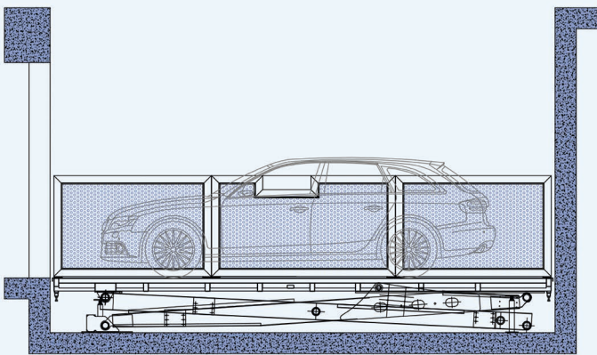
Section View-DOWN
